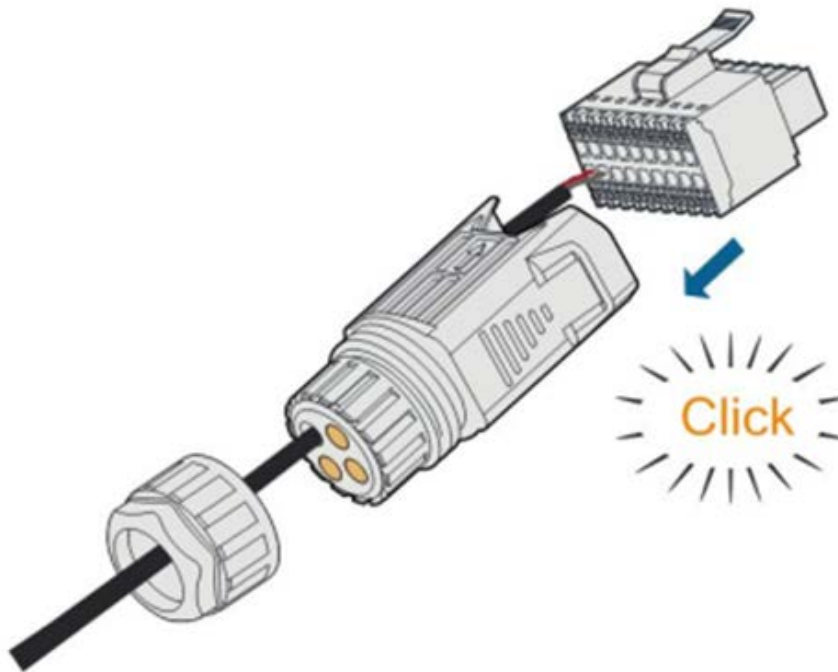
Diagram 4 – Assemble the multiplug
