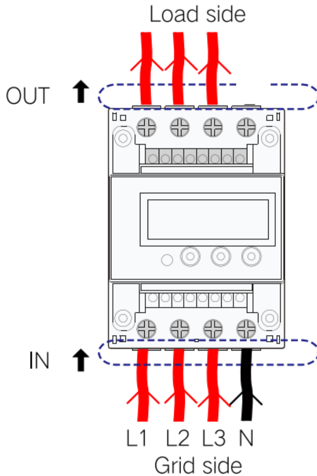
Diagram 2 – Electrical connections
