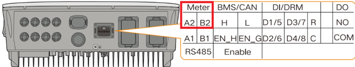
Diagram 3 – Meter connections on Multiplug
