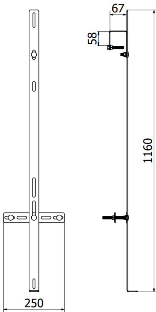
Fig.1 Dimensions of the structure
