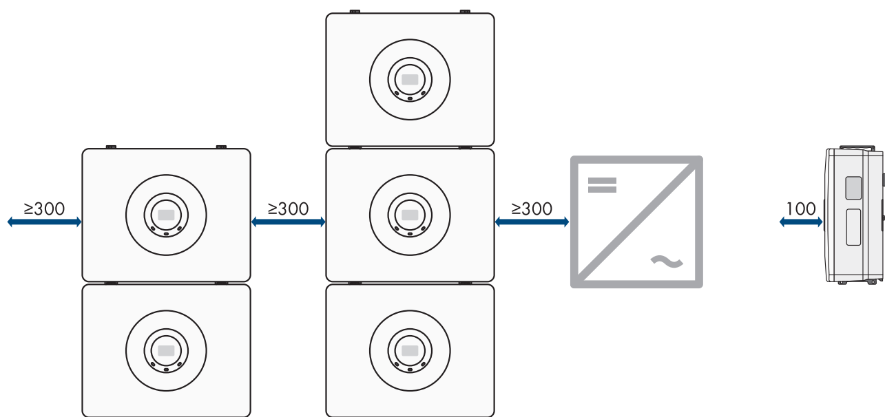
Figure 8: Recommended clearances (dimensions in mm)
