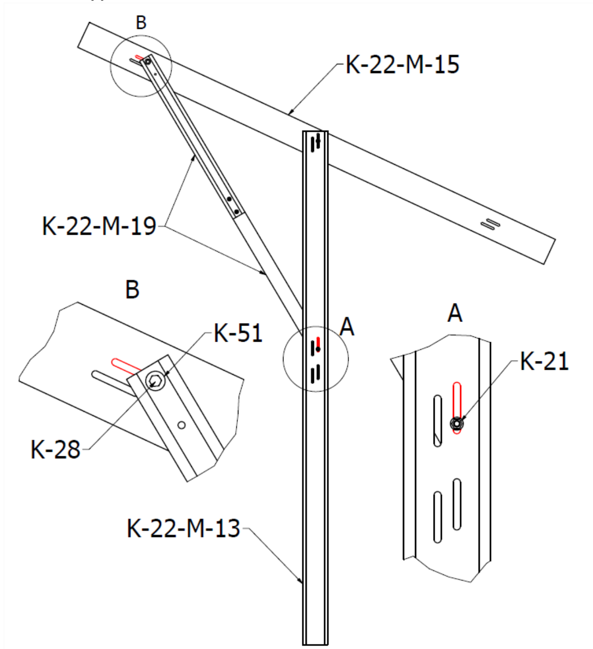
FIG. 8. Assembly of the longer arm to the main beam and support (projection I)
