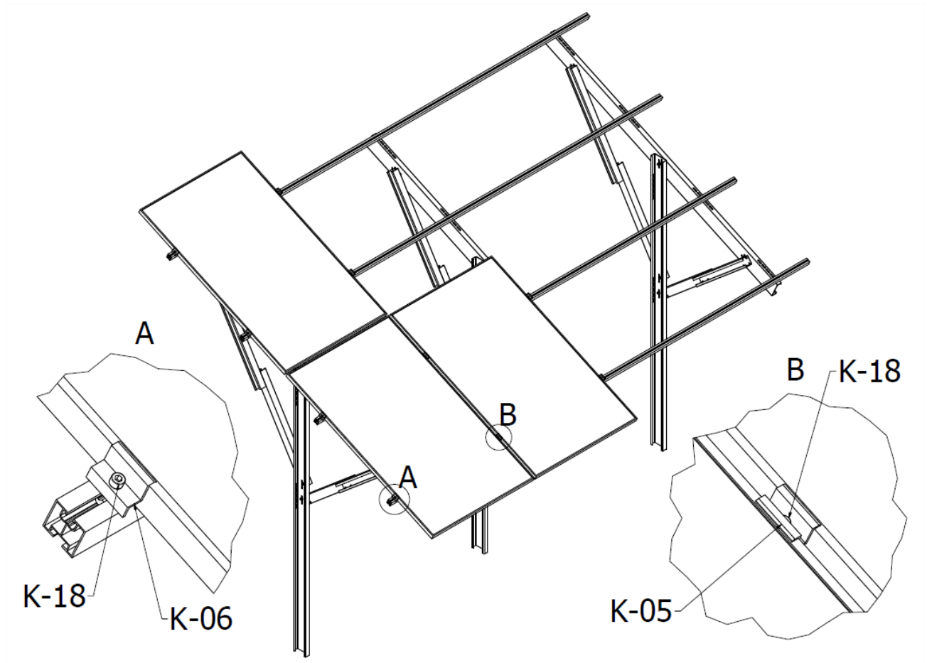
FIG. 18. Assembly of modules and mounting of K-05 and K-06 clamps
