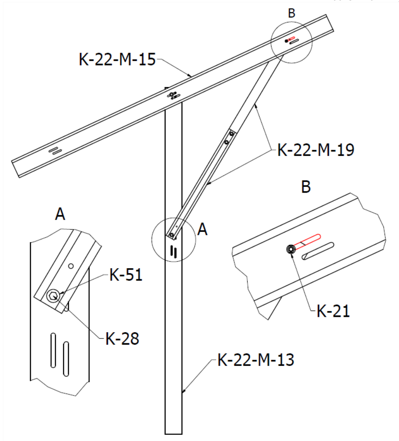
FIG. 9. Assembly of the longer arm to the main beam and support (projection II)
