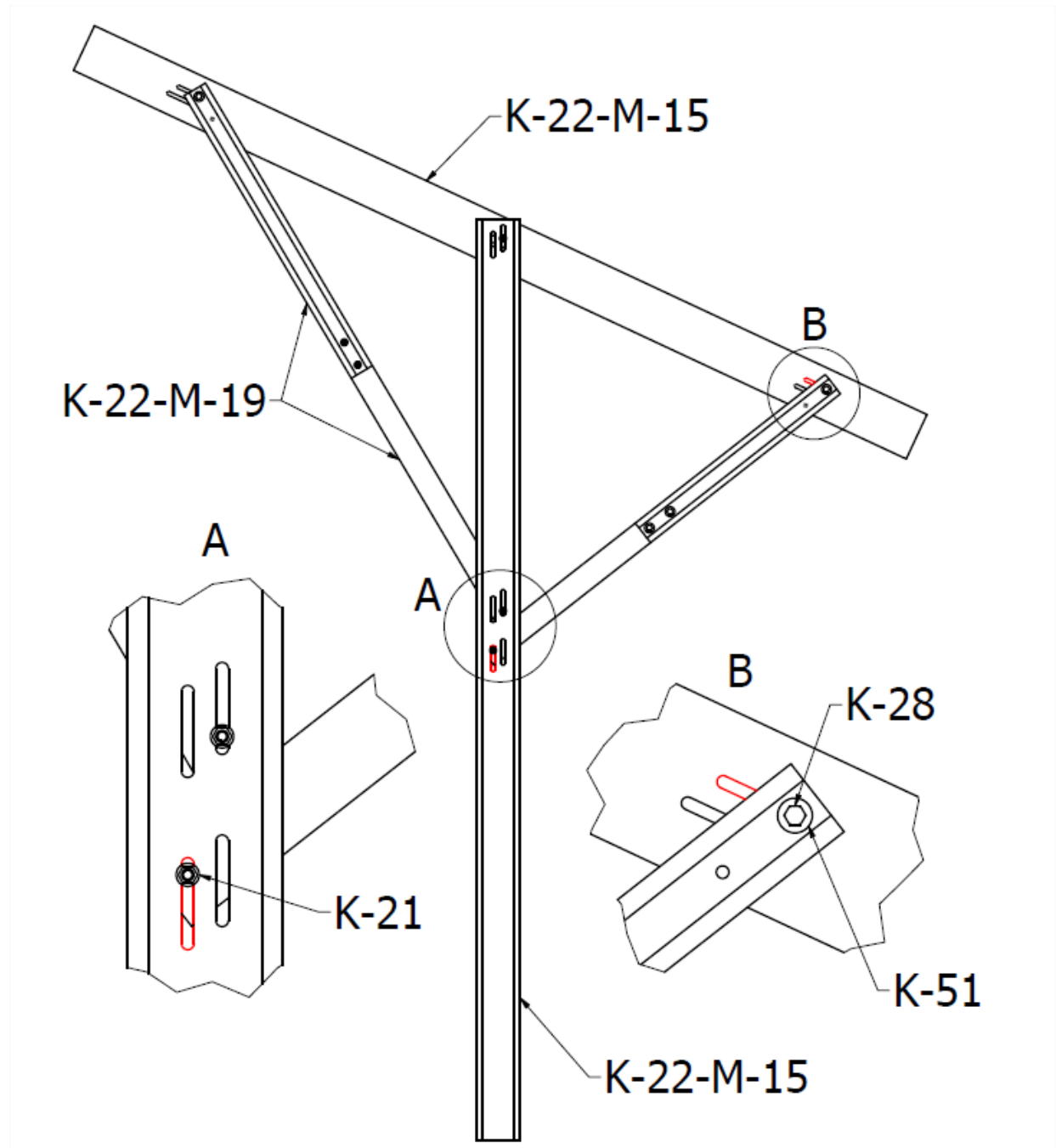
FIG. 10. Assemble the shorter arm to the main beam and support
