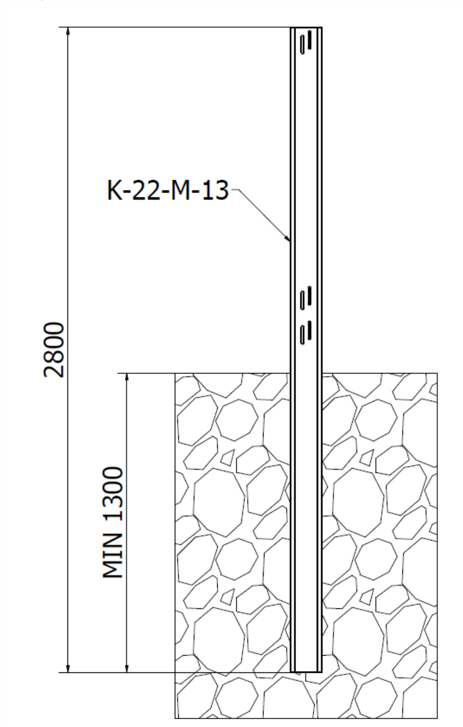
FIG.4. Installation of supports in the ground
