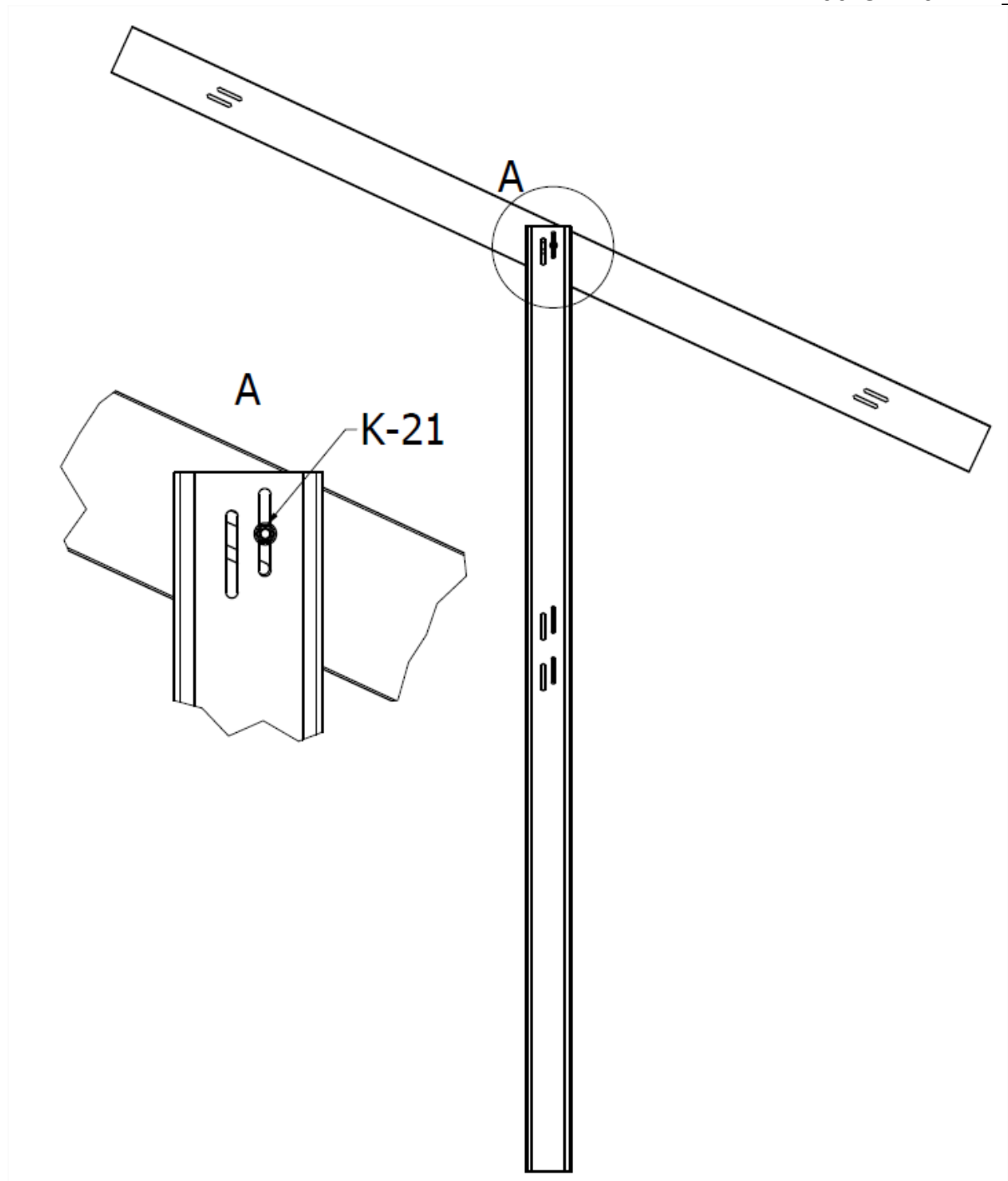
FIG. 6. Assembly of rafters with support (projection II)
