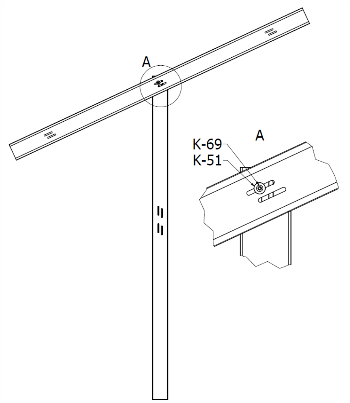
FIG.5. Assembly of rafters with support (projection I)
