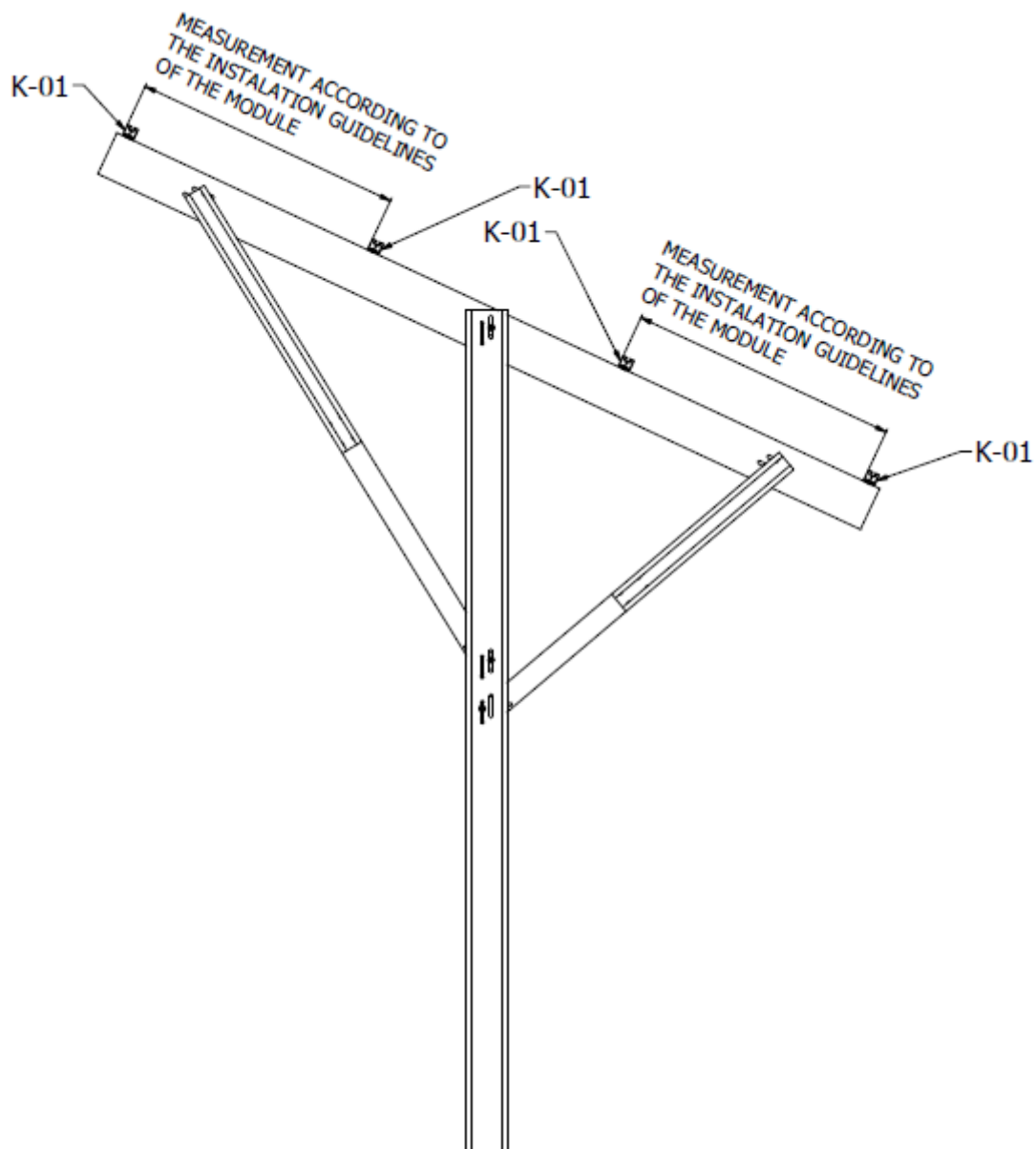
FIG.16. Spacing of K-01 mounting profiles
