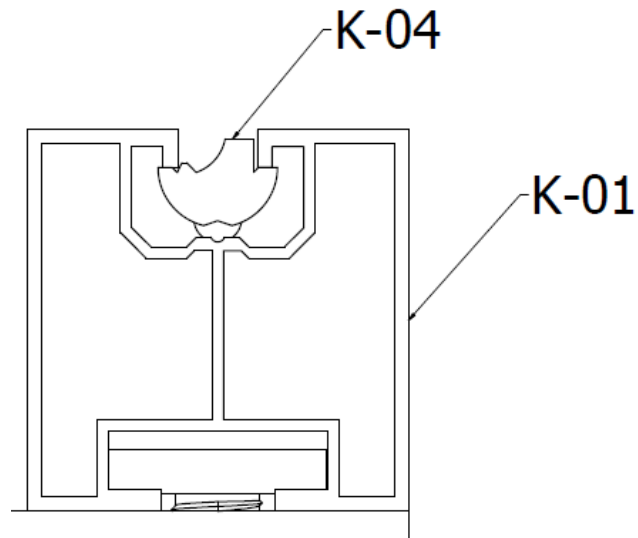
FIG. 17. Assembly of K-04 gully to K-01 profiles
