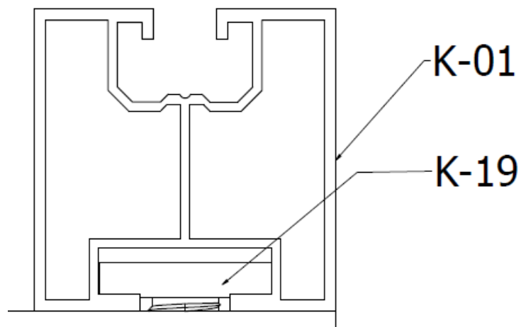
FIG. 15. Installation of K-01 profiles
