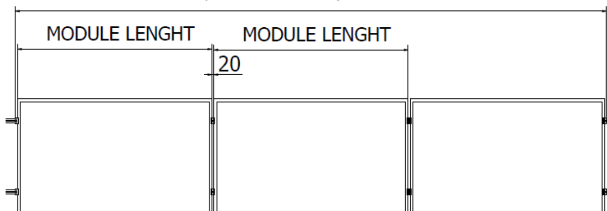
FIGURE. 2 Construction row length of short side mounted structures
