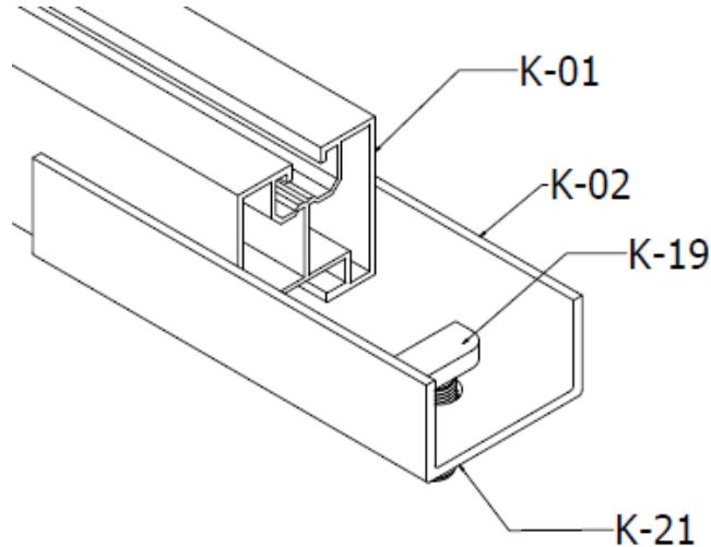
FIGURE. 7 Installation of the K-02 connector with the K-01 profile
