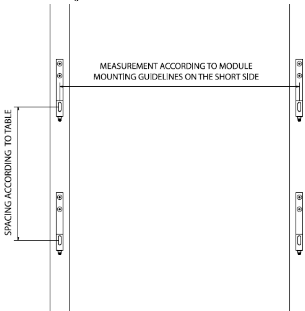
FIGURE. 5 Bracket spacing
