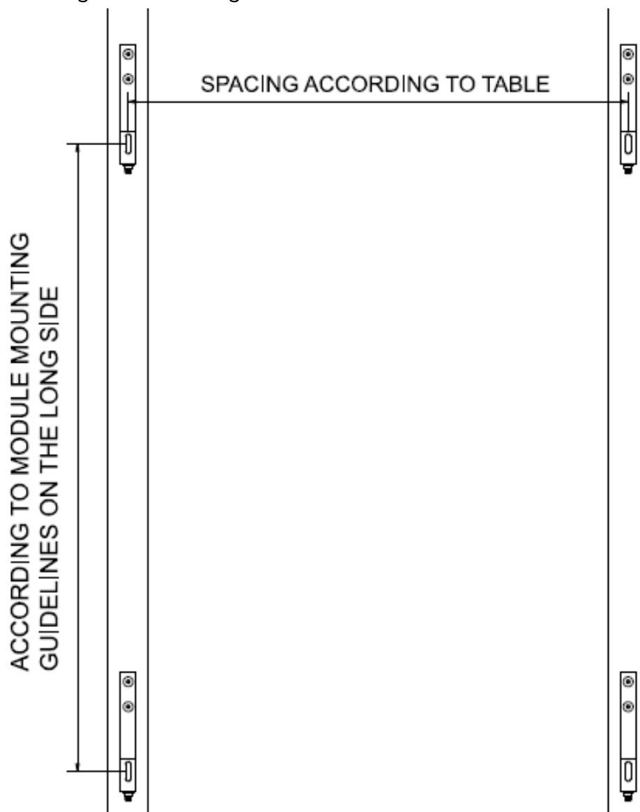
FIGURE. 4 Bracket spacing
