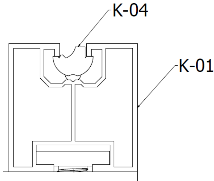
FIGURE. 11 Mounting of the K-04 t-slot nut to K-01 profiles
