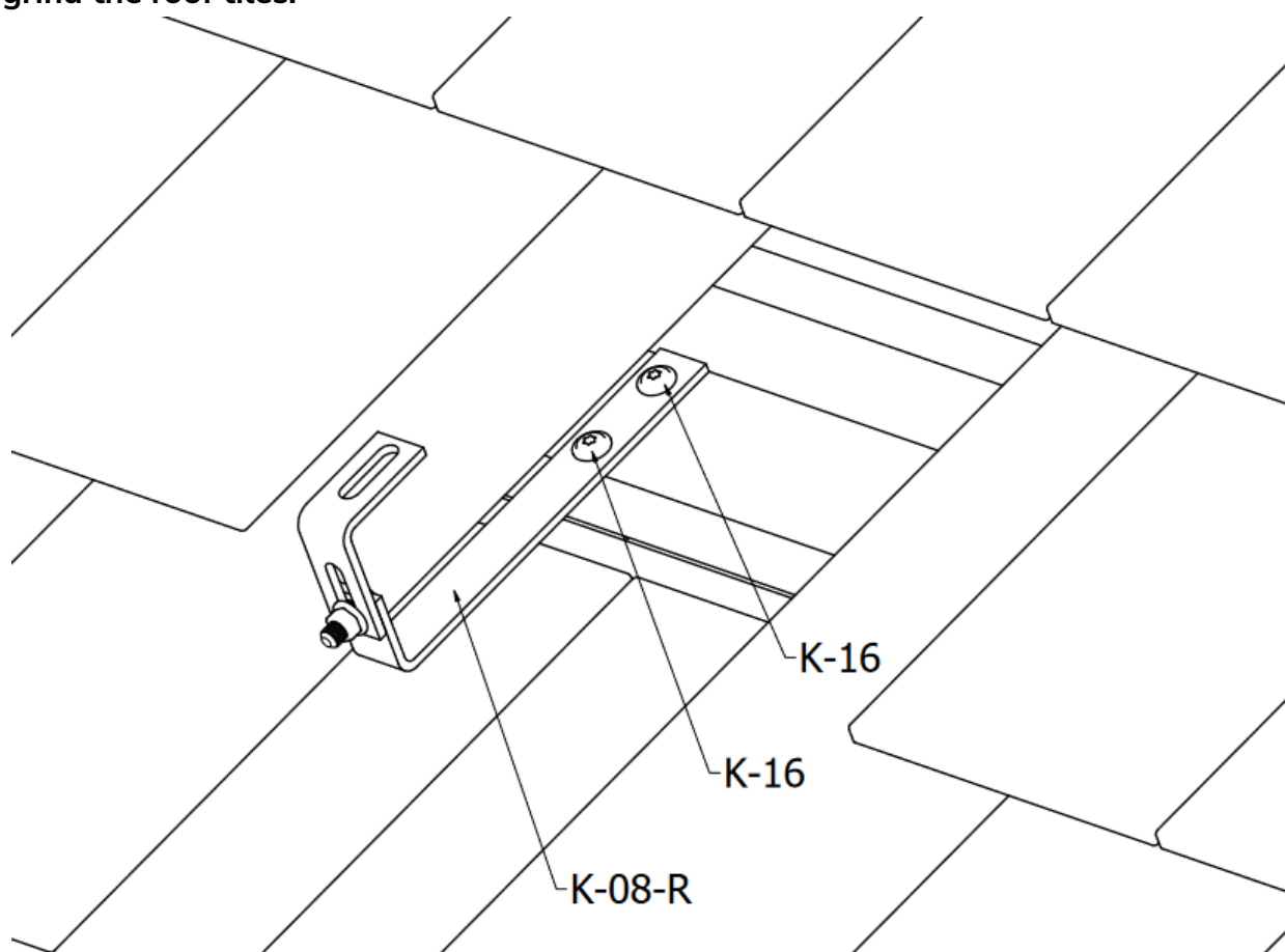
FIGURE. 6 Mounting of K-08-R hook
