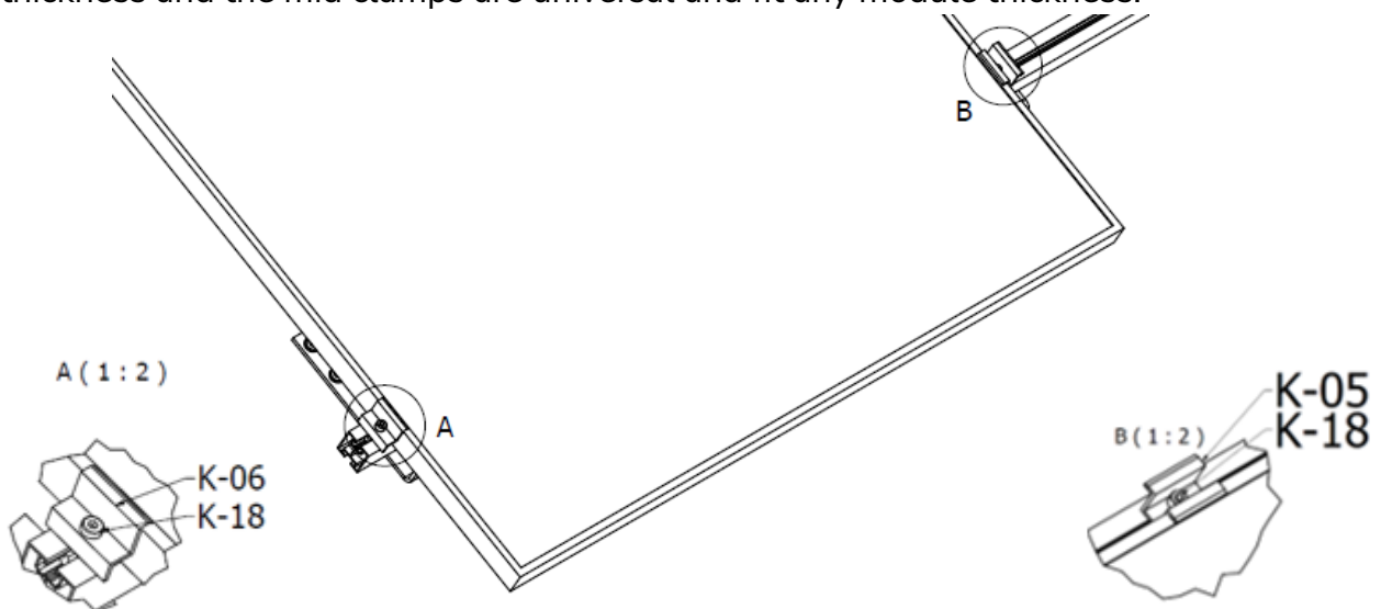
FIGURE. 12 Mounting of the modules and mounting of the K-05 and K-06 clamps
