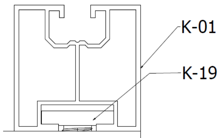
FIGURE. 9 Mounting of K-01 profiles
