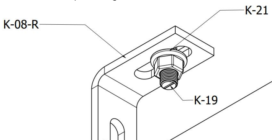
FIGURE. 10 Mounting of "T" bolts
