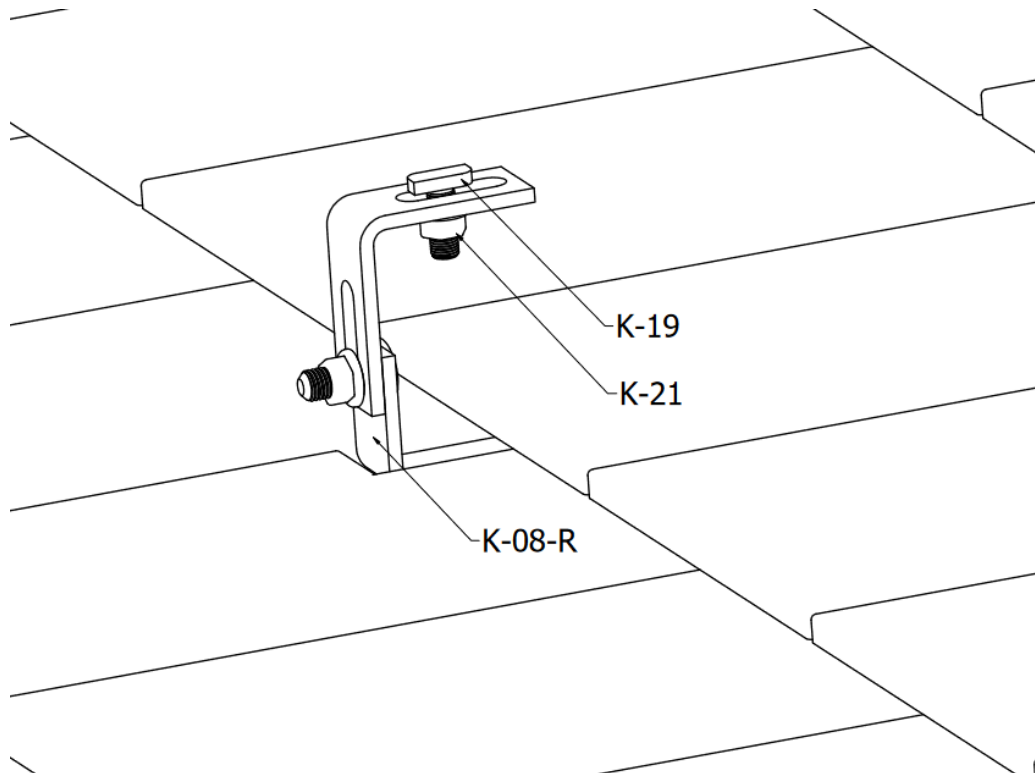
FIGURE. 8 Mounting of T-bolts v2.0 EN
